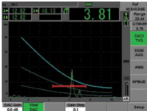
EPOCH 600 Dynamic DAC/TVG Feature
