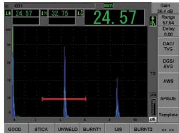
EPOCH 600 Template Storage Feature
