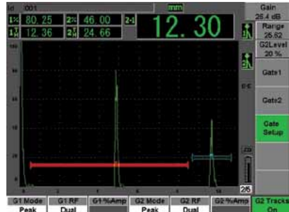
EPOCH 600 Echo to Echo with Gate Tracking
